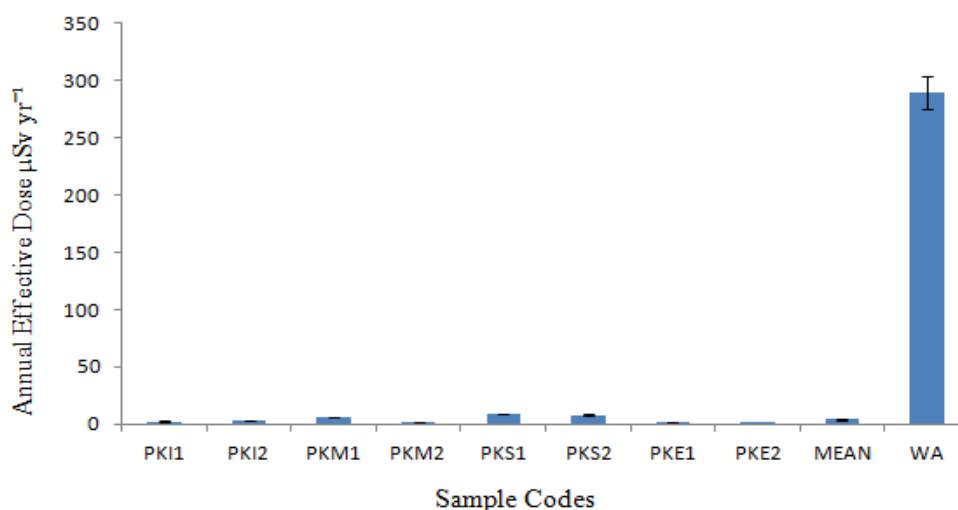
Fig. 3. Annual effective dose ( \mu\text{Sv yr}^{-1} ) of palm kernel oil WA: World Average Value [7]
