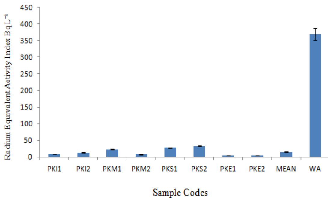
Fig. 4. Radium equivalent activity index ( \text{Bq L}^{-1} ) in Palm Kernel Oil WA: World Average Value [7]
